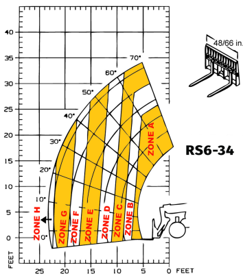
Load Chart Other Imperial
